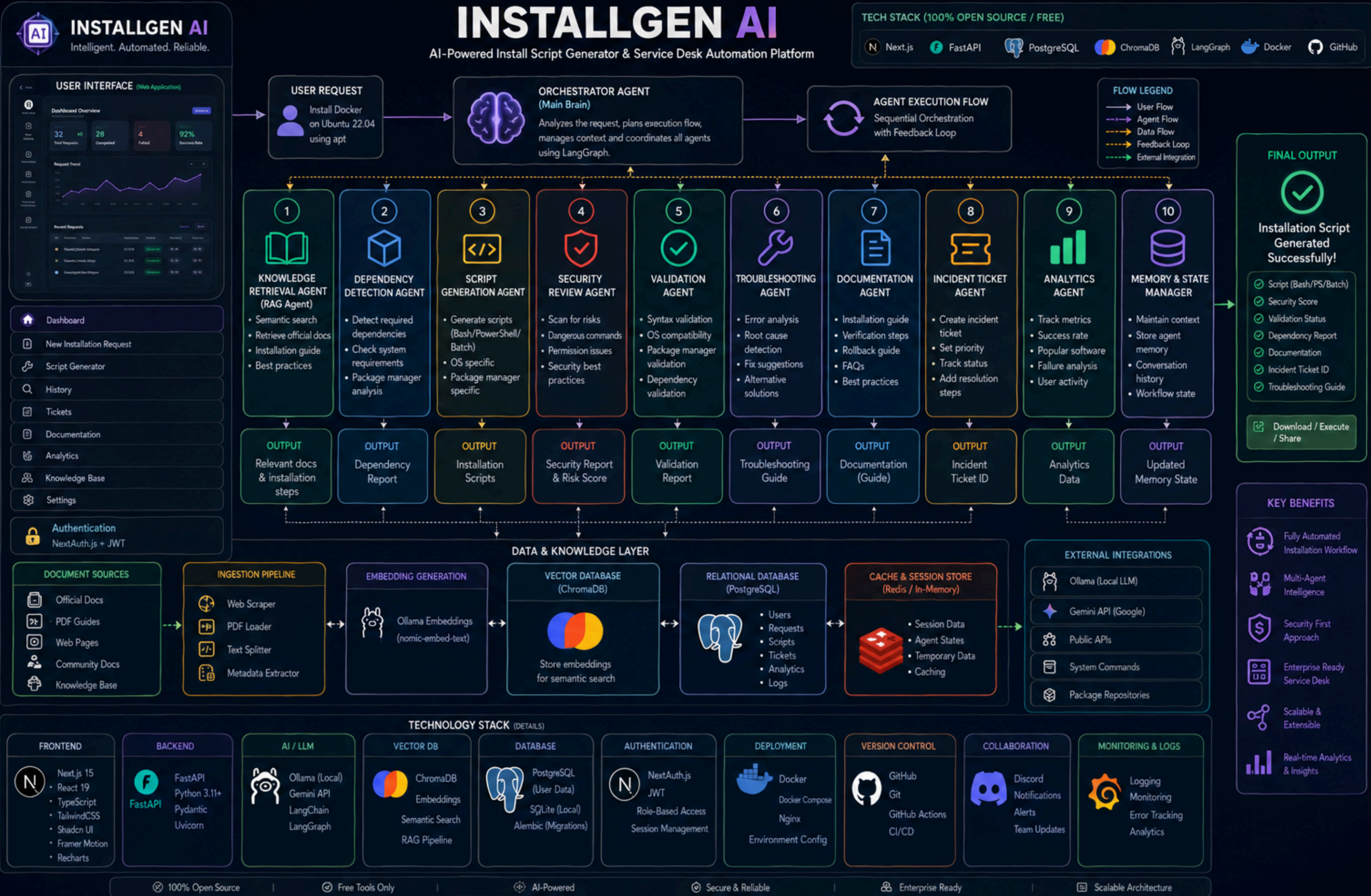
workflow architecture of installgen-AI
